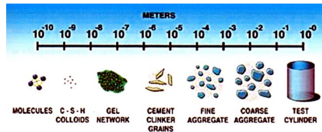
Fig. 1.2 Particle Size Scale
