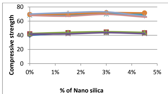
Fig :Durability Compressive Strength Test Base Attack
