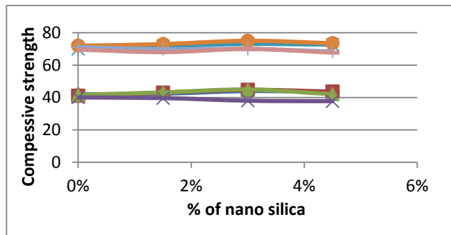
Fig :Durability Compressive Strength Test Acid Attack
